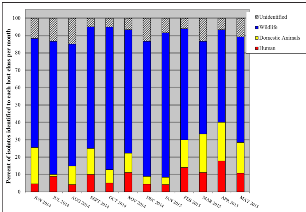
Figure 6.13. Three-way split of E. coli source class identifications by month for all stations combined
