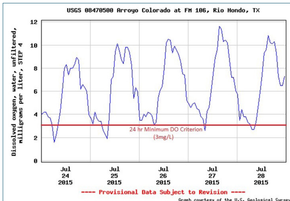
Figure 4.2. 24-hour data collected within the DO Zone of Impairment
