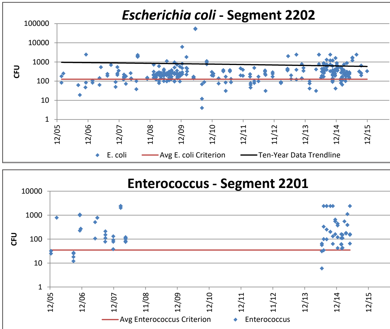
Figure 4.10. E. coli and Enterococcus concentrations in the Arroyo Colorado
