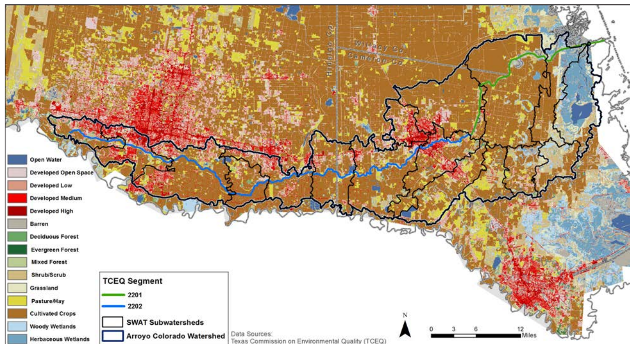
Figure 2.5. Land cover map
