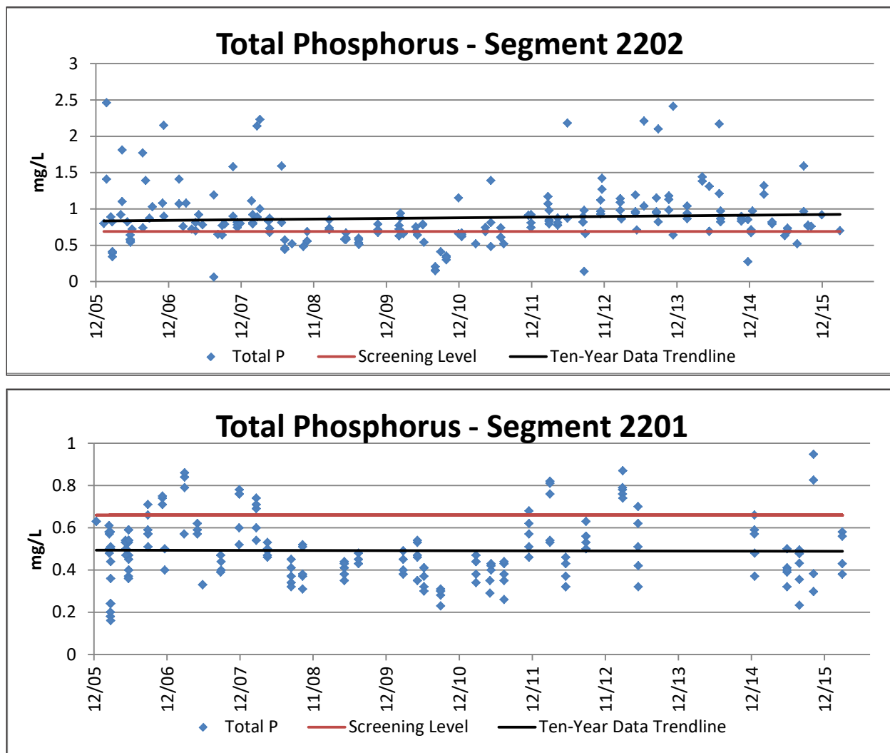
Figure 4.7. Total phosphorus concentrations in the Arroyo Colorado
