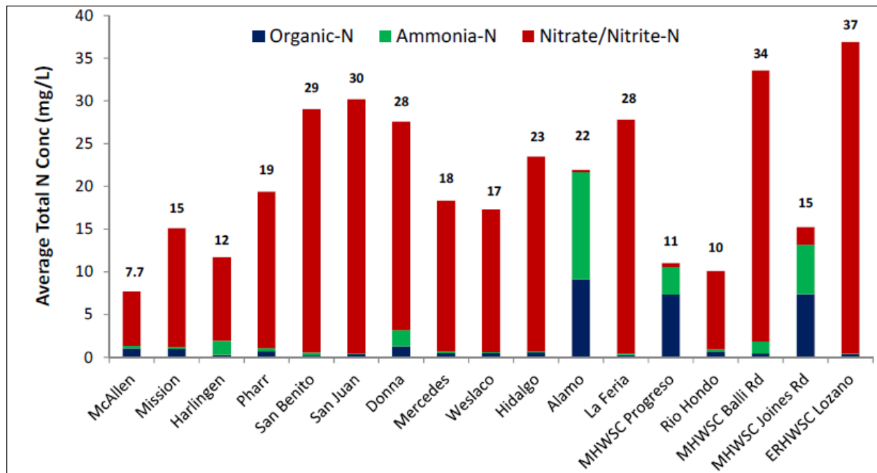
Figure 5.4. Average WWTF effluent TN concentrations, from September 2010 to August 2011
