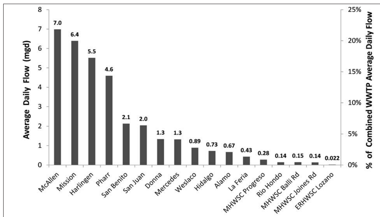
Figure 5.3. Average daily effluent flows (left axis) and corresponding percentages of the combined effluent flow (right axis) for all 17 WWTFs, from September 2010 to August 2011
