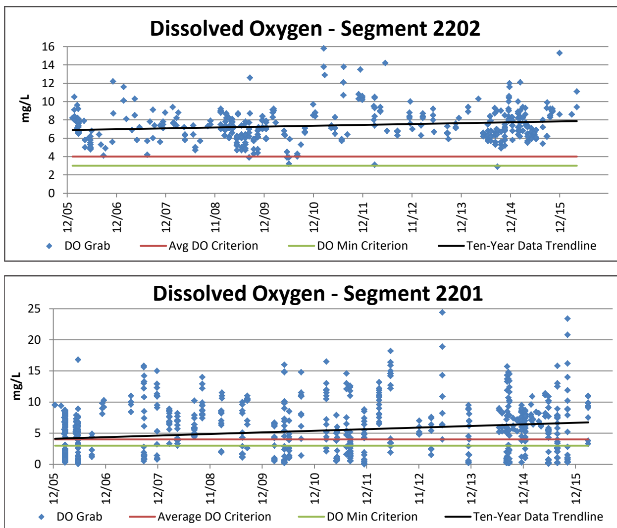
Figure 4.4. DO time series data for Segments 2202 and 2201
