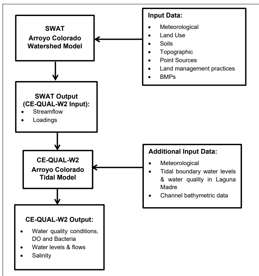
Figure 9.1. Schematic of modeling system
