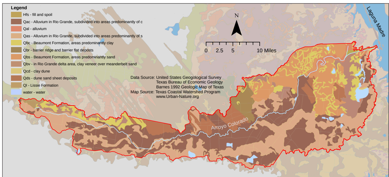
Figure 2.3. Surface geology in the Arroyo Colorado watershed (Arroyo Colorado WPP 2007)
