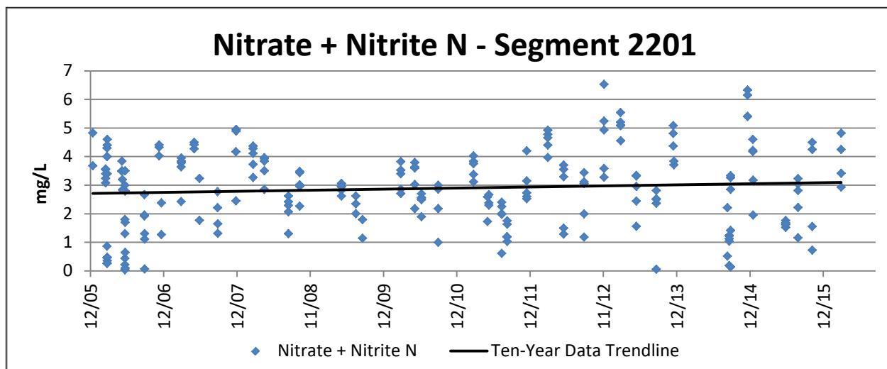
Figure 4.5. Nitrate + Nitrite-nitrogen concentrations in the Arroyo Colorado
