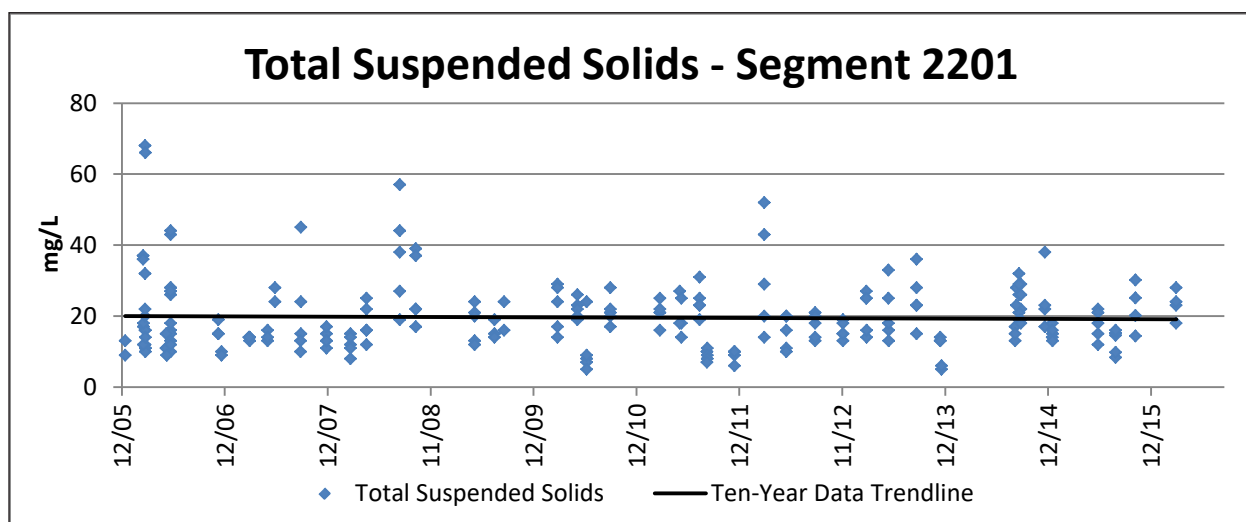
Figure 4.9. Total suspended solids concentrations in the Arroyo Colorado
