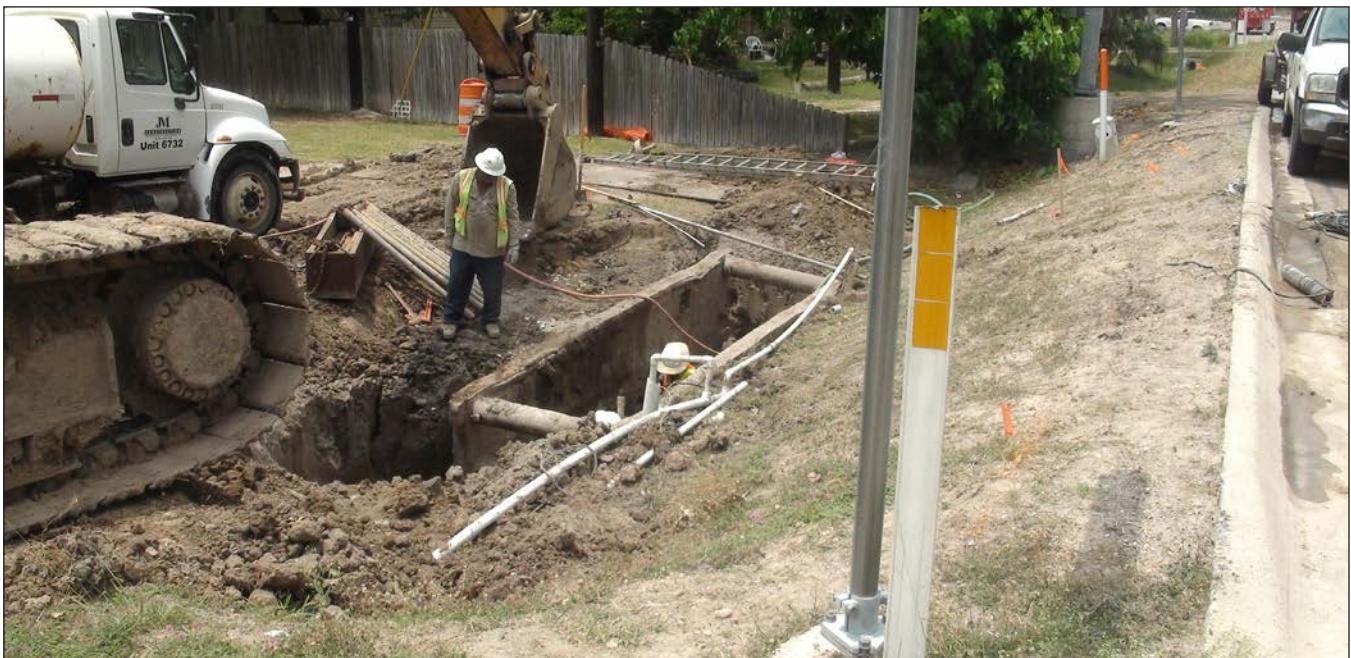
Shoring and dewatering of excavated trench to install sanitary sewer line and manhole, La Feria, TX
