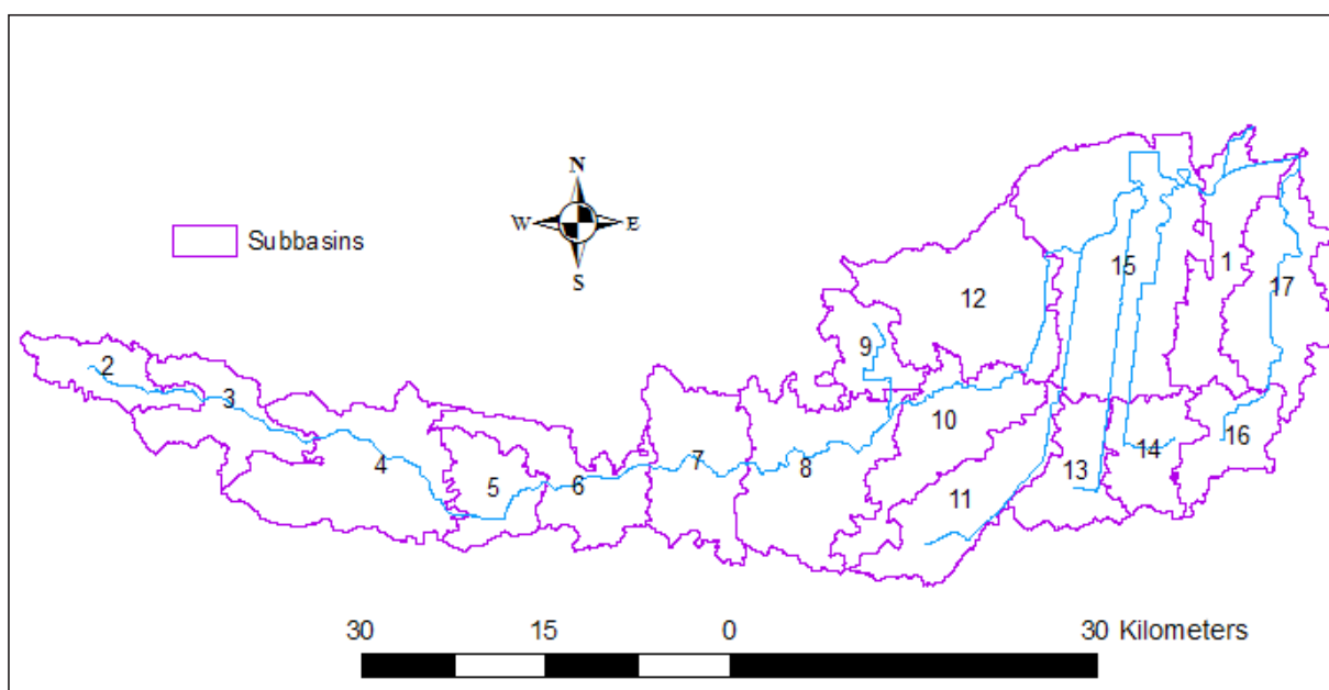
Figure 6.1. Arroyo Colorado subbasins used by SWAT
