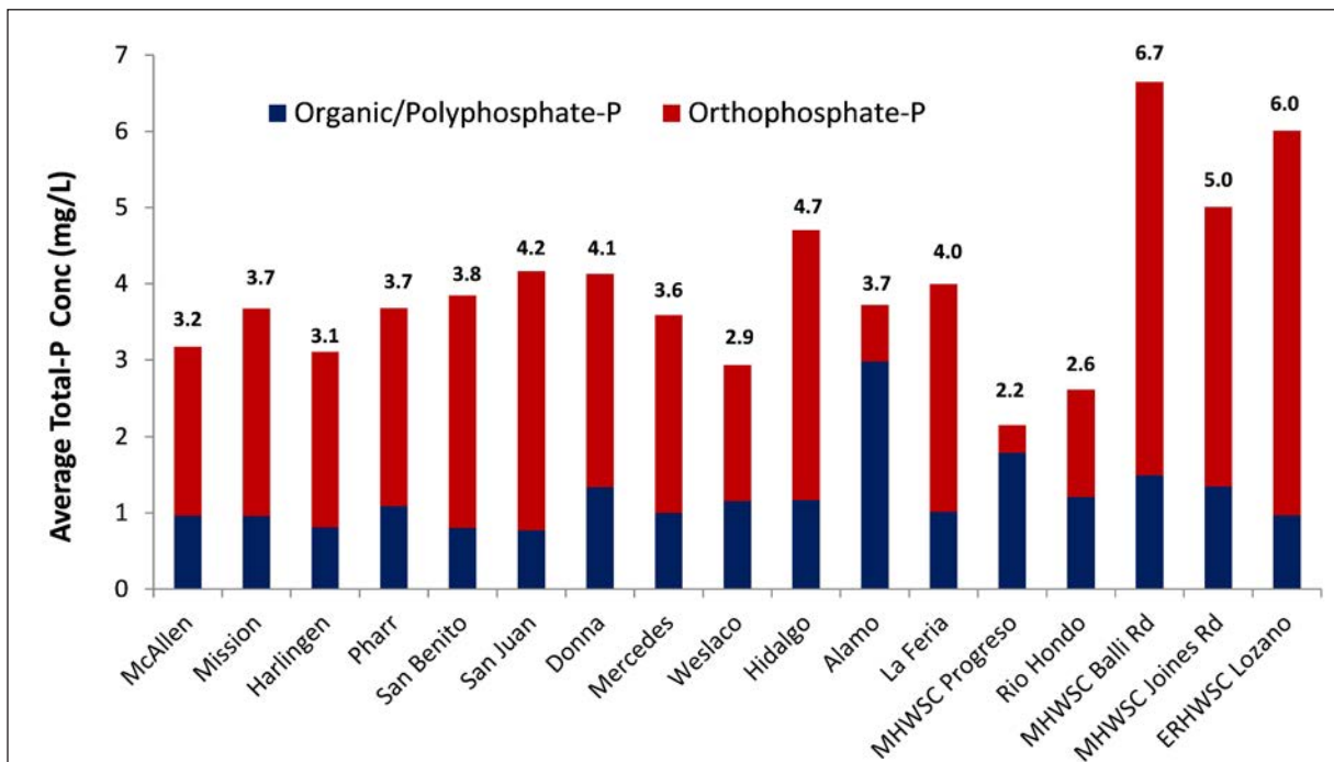
Figure 5.7. Average WWTF effluent total-P concentrations for the 46-week sampling period
