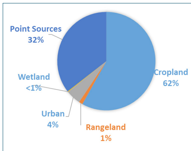
Figure 6.4. Predominant sources of nitrogen loads in the Arroyo Colorado watershed
