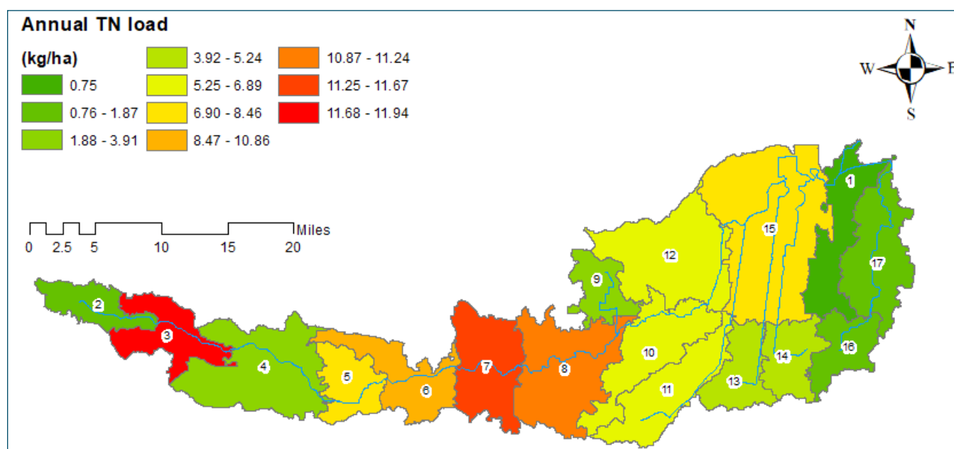
Figure 6.5. Estimated total nitrogen export (kg/ha) from upland nonpoint sources by subbasin
