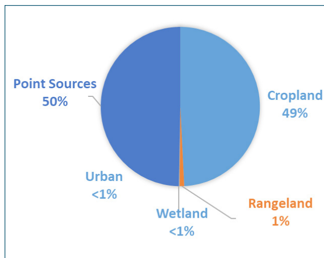
Figure 6.6. Predominant sources of phosphorus in the Arroyo Colorado watershed
