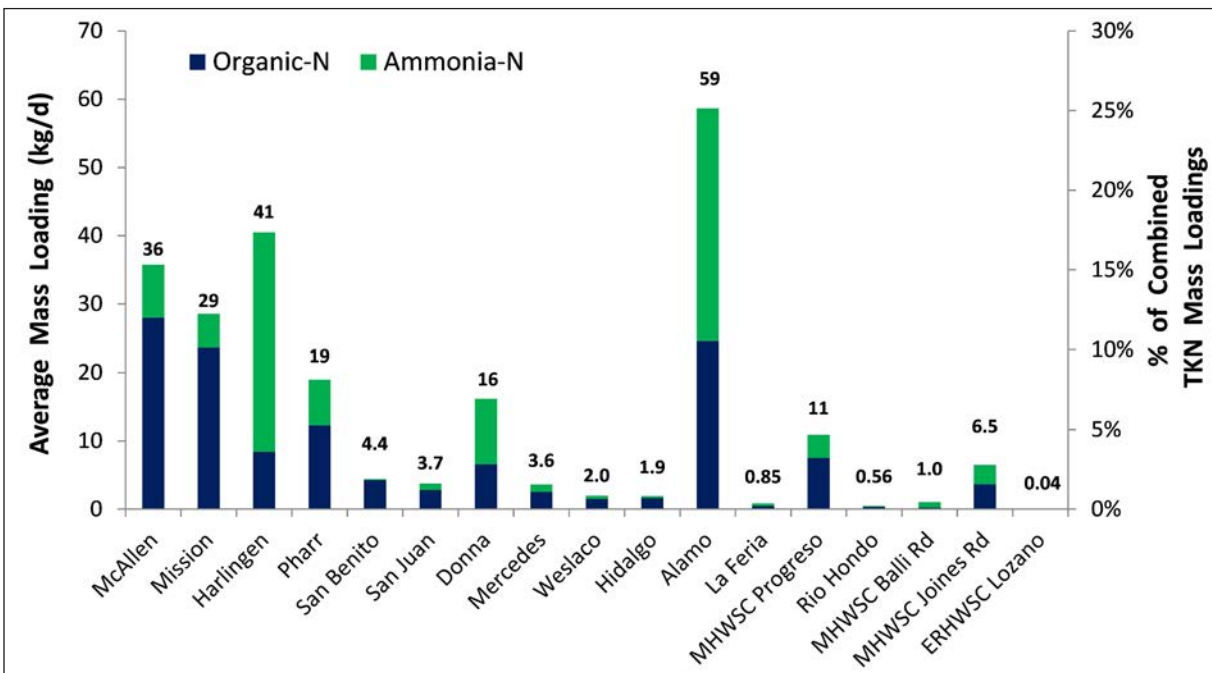
Figure 5.6. Average WWTF effluent TKN mass loadings (i.e., the sum of the organic-N and ammonia-N loadings), from September 2010 to August 2011
