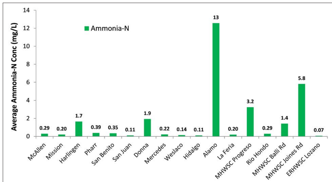
Figure 5.5. Average WWTF effluent ammonia-N concentrations, from September 2010 to August 2011
