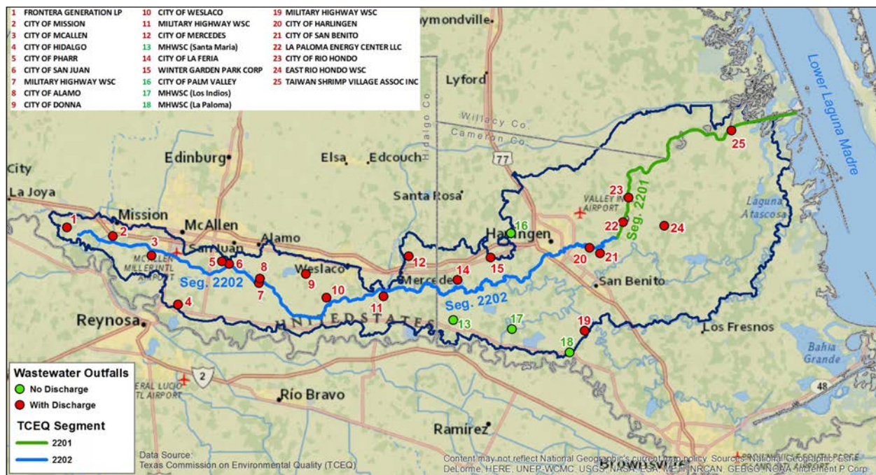
Figure 5.2. Permitted wastewater outfalls within the Arroyo Colorado watershed
